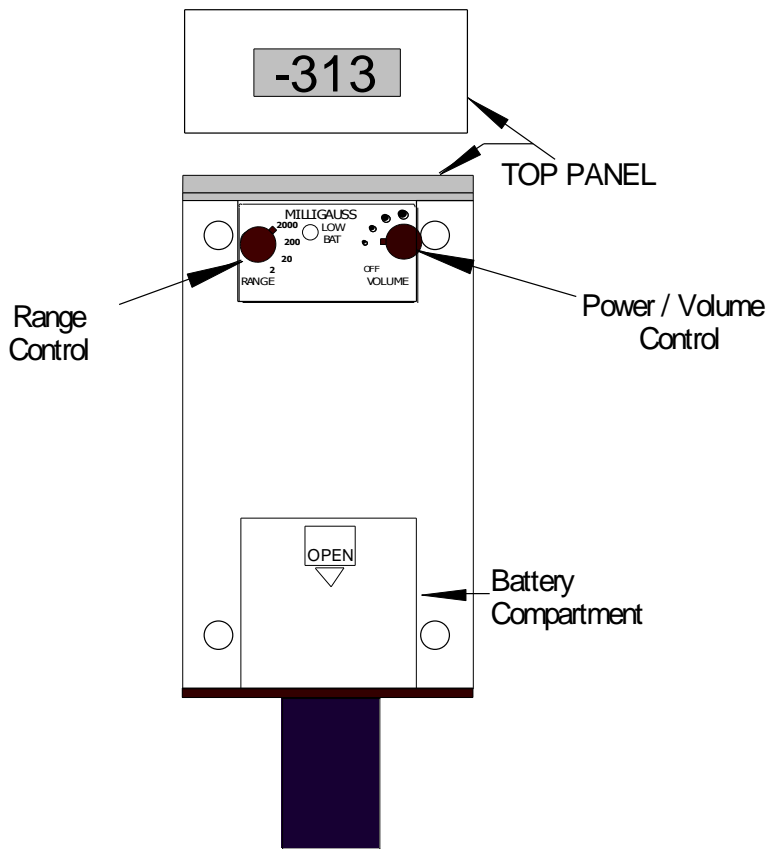
Figure 2, Instrument Controls
